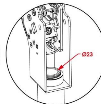
Spigot Inner Diameter
